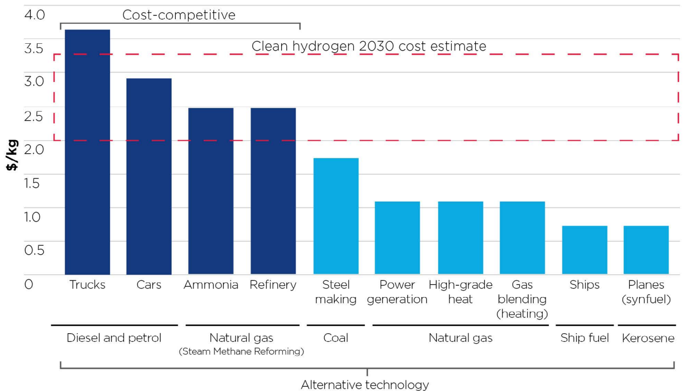
Figure 10 Breakeven cost of hydrogen against alternative technology for major applications in 2030. 35
